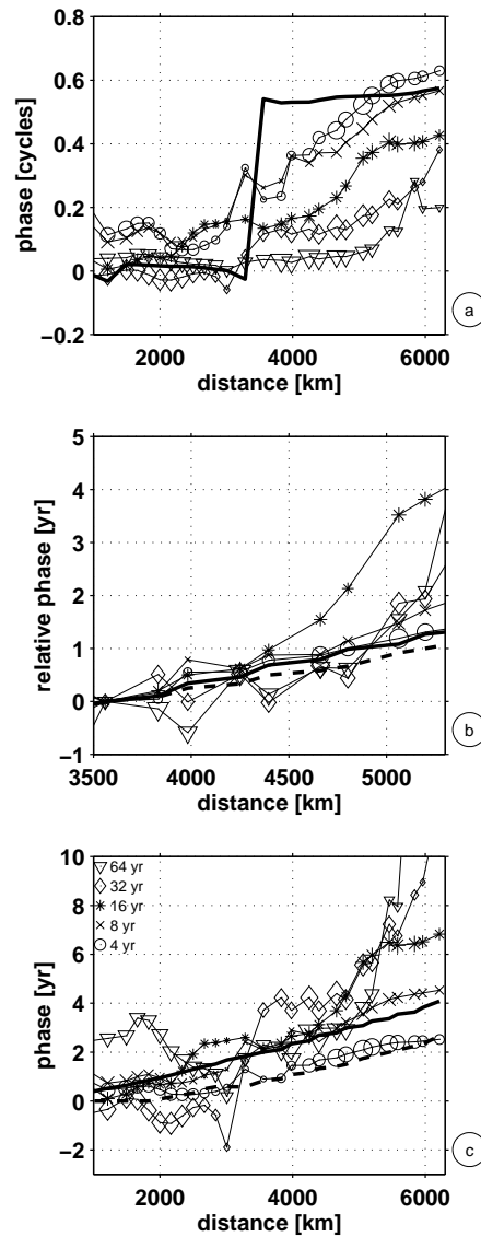
Figure 8. Phases of the harmonic variation of the upper 440 m heat content relative to the forcing both in phase-distance and time-distance space. The phase-distance diagram (a) includes the phases of the heat content anomalies for the mixed layer model run with a forcing period of 16 years (solid line in a). The time-distance diagrams (b and c) also include the graphs for the spreading of the maximum tracer concentration of experiment TRACER (dashed) and the propagation time calculated directly from the model's currents (solid). The time-distance diagram (b) displays a part of full pathway (c) in which advective spreading of the anomalies is dominant.
