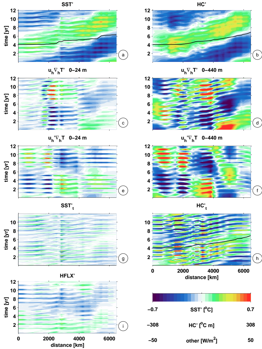
Figure 4. Sea surface temperature and upper 440 m heat content anomalies of the experiment NAO-D12 along the pathway of the NAC (graphs a and b), their tendency (graphs g and h), and components contributing to their tendency. Shown is always one full cycle of the forcing. To make the SST tendencies in the graphs c, e and g comparable to the heat content change and the surface heat flux it has been assumed that the temperature change in the uppermost model layer is representative of the mixed layer, here assumed to be three times as thick as the uppermost layer (i.e. 72 m). The black lines in graphs a, b and h show how a tracer patch inserted at the beginning of the pathway propagates along the pathway.
