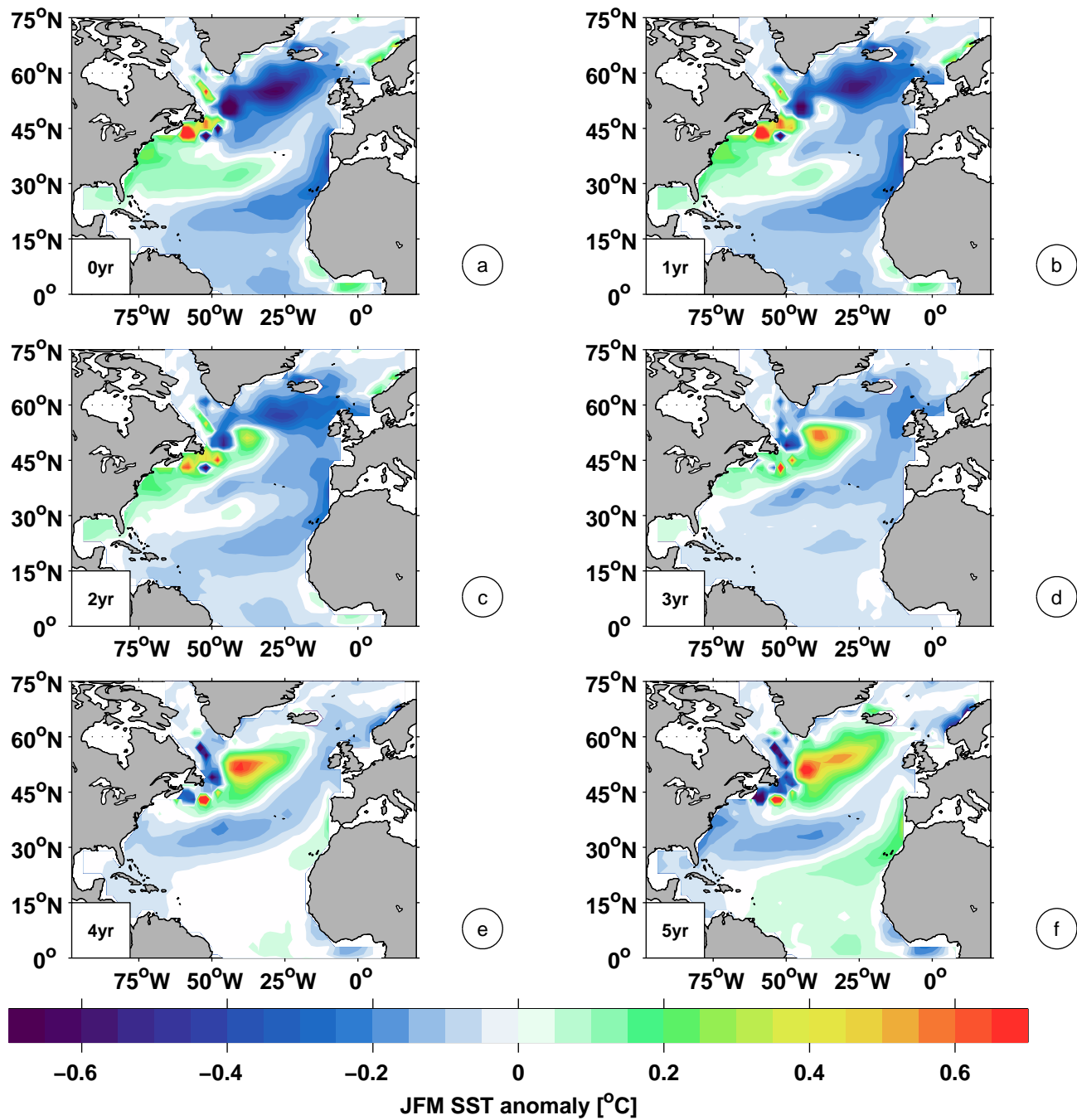
Figure 2. Sea surface temperatures of the experiment NAO-D12 zero, one, two, three, four, and five years after the sinusoidal forcing modulation started from zero. In response to the idealized wind and windstress anomalies a temperature anomaly is formed off the North American east coast. This anomaly apparently propagates along the pathway of the NAC.
