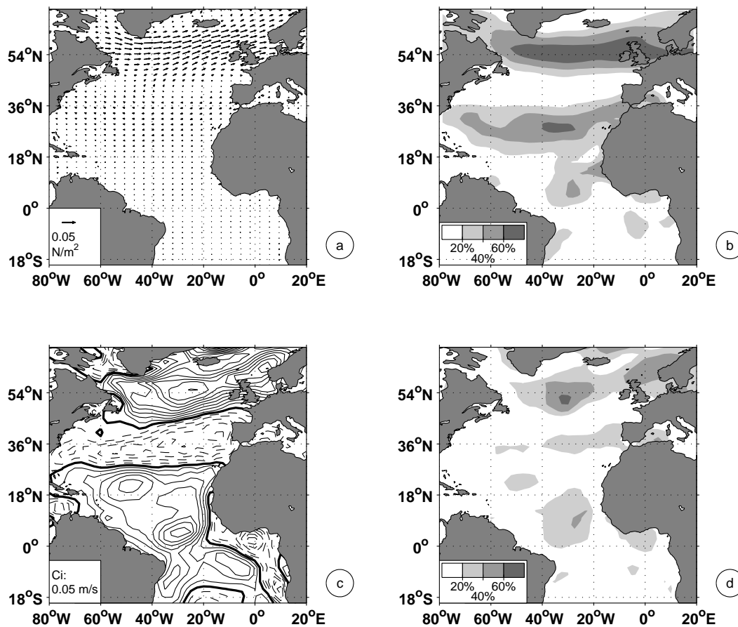
Figure 1. Wind stress (a) and wind speed (c) forcing anomaly fields used for the experiments. The anomaly fields have been derived by regressing the wind stress and wind speed of the NCEP/NCAR Reanalysis onto the NAO time series. The two displays on the right show the fraction of the total variance explained by the NAO-regressed anomalies for the zonal component of the wind stress (b) and the wind speed (d), respectively. For all calculations winter averages (November to April) have been used.
