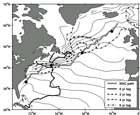
Figure 3. Lagged correlations of monthly SST anomalies for the 12 year idealized NAO period. The lagged correlations are calculated similarly to those of Sutton and Allen [1997], using the SSTs in the area 31 to 39°N and 60 to 80°W as reference. We did, however, not apply a three year running mean filter to our modeled data. Contoured is a correlation of 0.75. Also shown is the NAC's pathway as used in our analyses. The filled circles denote 0, 2000, 4000, and 6000 km distance from the beginning of the pathway.
