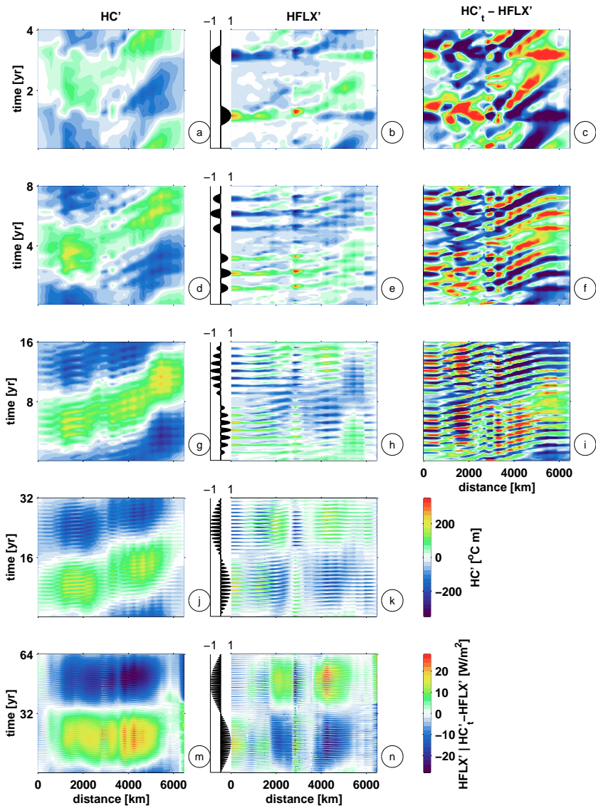
Figure 5. Upper ocean heat content, surface heat flux and oceanic heat transport divergence for selected NAO periods. Shown is again one full cycle of the sinusoidal forcing. The forcing modulation is displayed between first and second column. The heat transport divergence has been determined by subtracting the surface heat fluxes from the total heat content changes.
