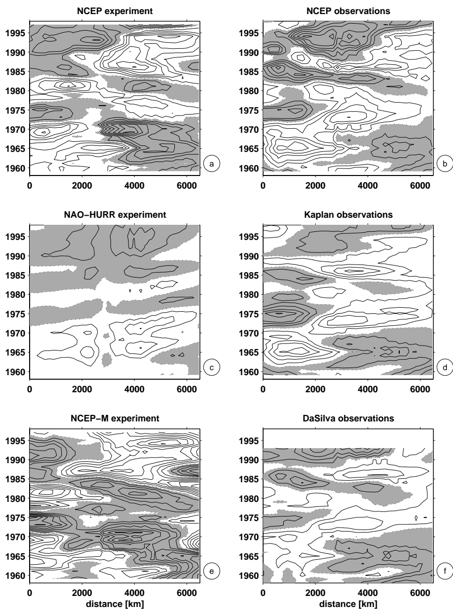
Figure 9. Hovmuller diagrams of the wintery (NDJFMA) temperature anomalies along the NAC for the experiments NCEP (a), NAO-HURR (c), and NCEP-M (e) and for the observational data sets NCEP (b), Kaplan (d) and DaSilva (f). Contour-interval is 0.2^\circ , shaded areas denote positive anomalies. A three year running mean has been applied to all data sets as has been done by Sutton and Allen [1997].
