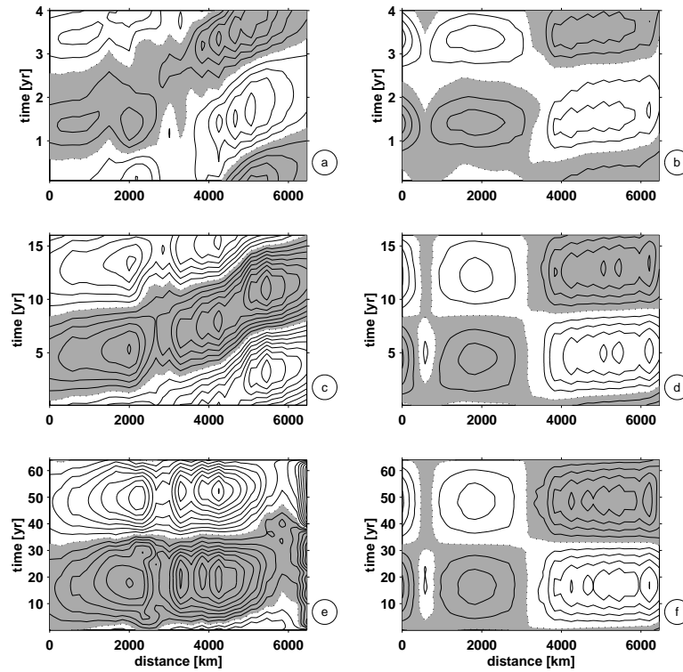
Figure 6. Heat content anomalies along the NACs pathway for the advective (left column, NAO-D) and non-advective (right column, NAO-M) ocean. Shown are forcing periods of 4, 16, and 64 years. The data has been filtered to remove the seasonal cycles. Contour interval is 0.05^{\circ}\text{C} , positive anomalies are shaded. While for the short period the response is somewhat similar between advective and non-advective ocean, the response for the long period shows no resemblance at all.
