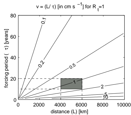
Figure 7. This diagram shows the propagation speed which is necessary to obtain maximal response for any given length- and timescale of the forcing. The realistic range for the NAC marked by the shaded area.
