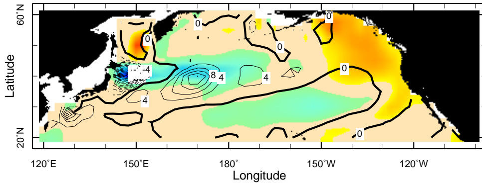
(B) OGCM SST(colors) Barotropic Transport(contours)
