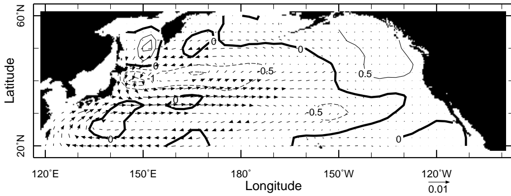
(B) OGCM SST(contours) Barotropic Current(vectors)
