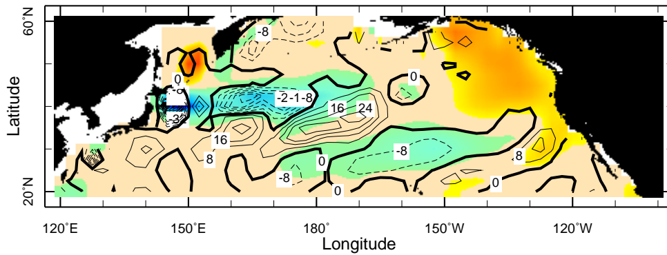
(C) OGCM SST(colors) Slow Baroclinic Transport(contours)
