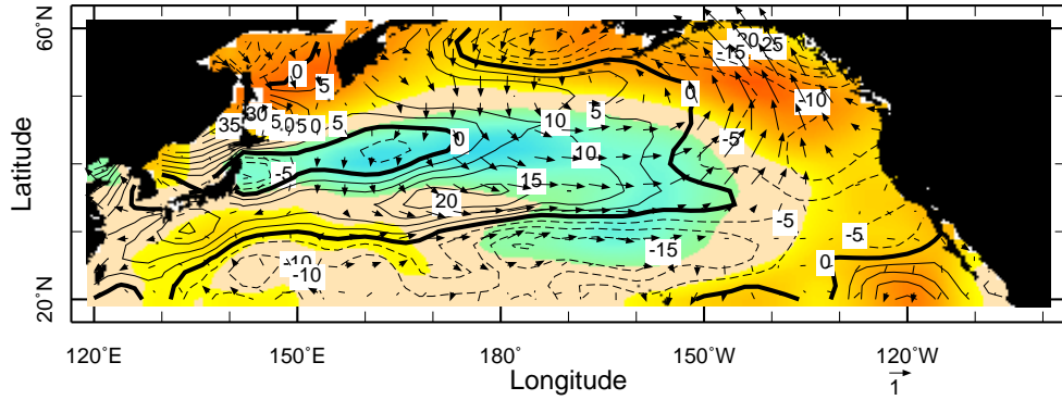
(A) DaSilva SST(colors) Heat Flux(contours) Winds(vectors)
