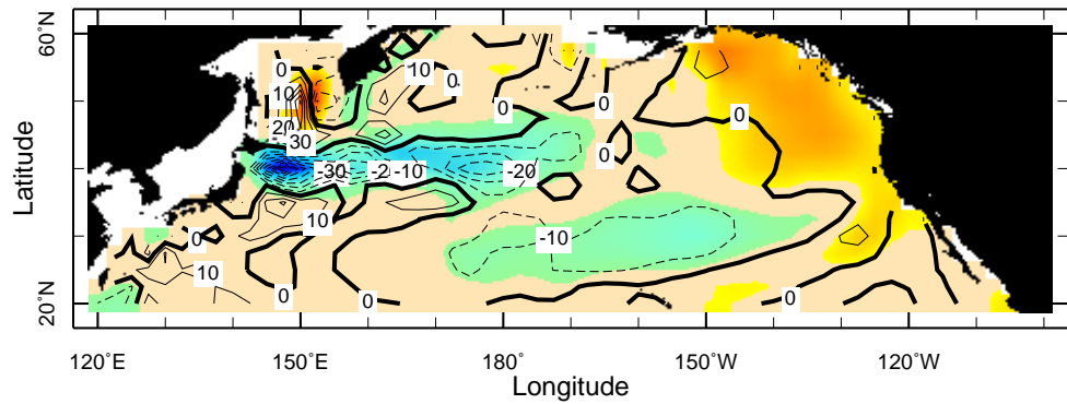
(C) OGCM SST(colors) Total Heat Transport(contours)
