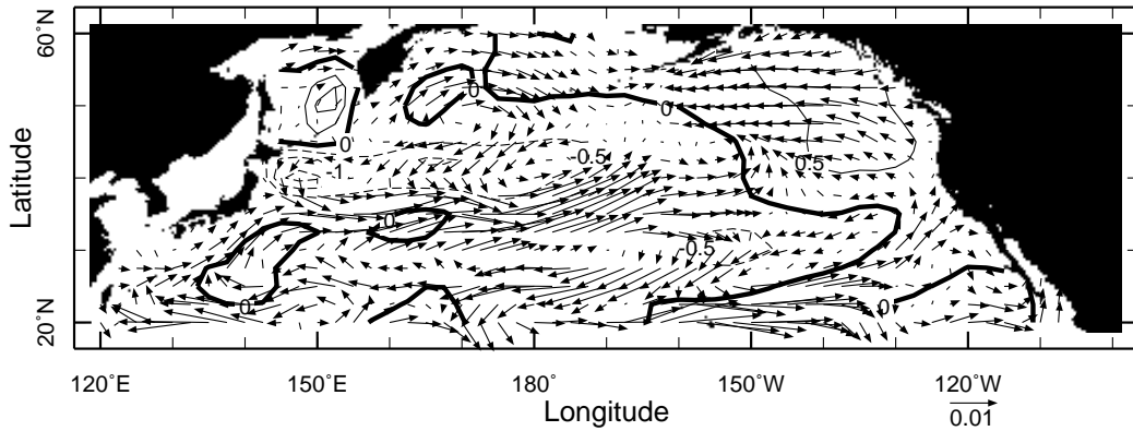
(C) OGCM SST(contours) Slow Baroclinic Current(vectors)
