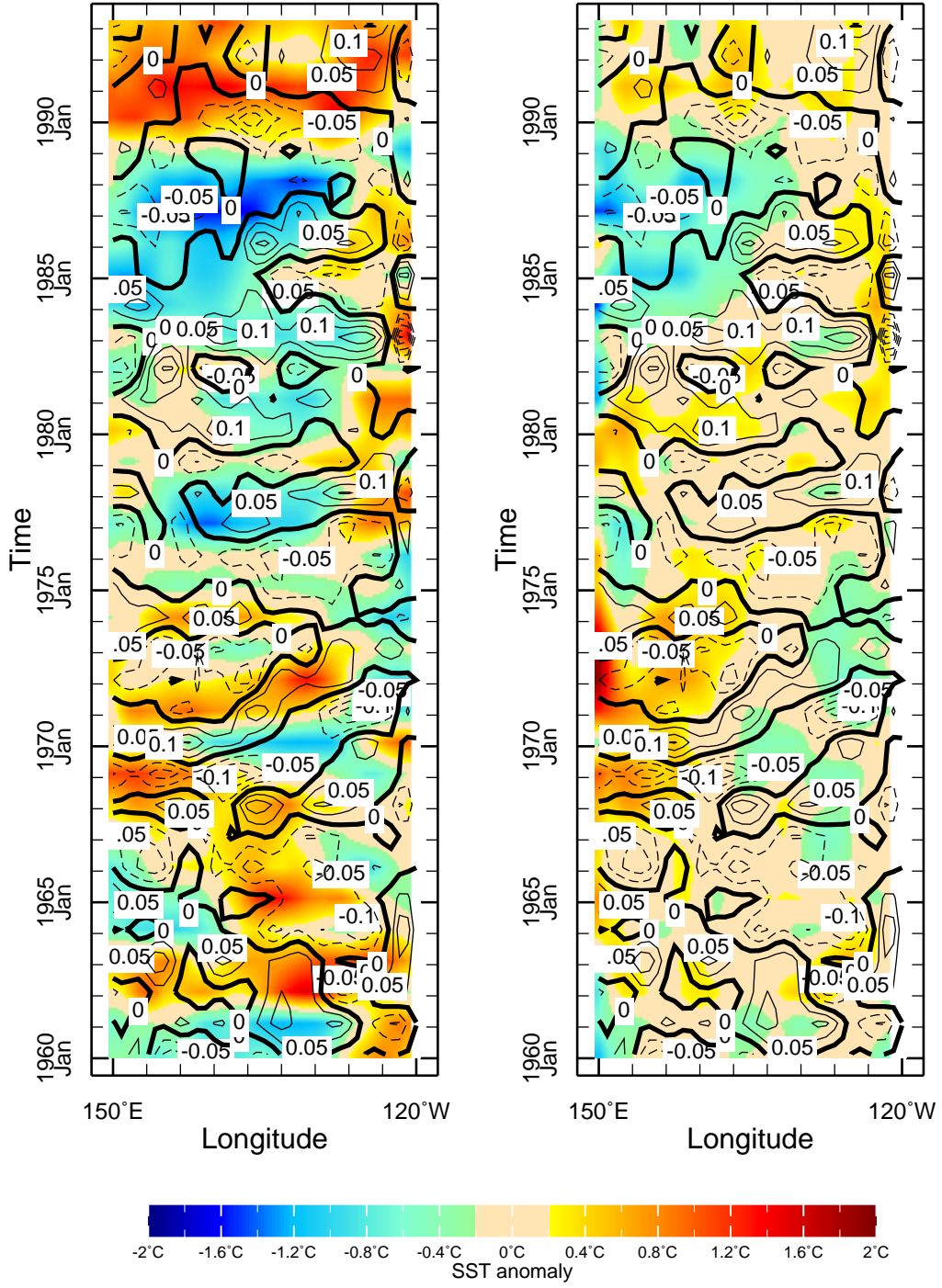
JFM SSTA and Curl of Wind Stress at 40N (A) DaSilva (B) OGCM
