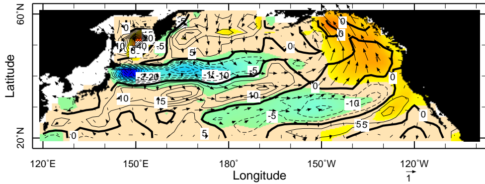
(B) OGCM SST(colors) Heat Flux(contours) Winds(vectors)
