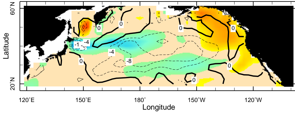
(A) OGCM SST(colors) Ekman Transport(contours)
