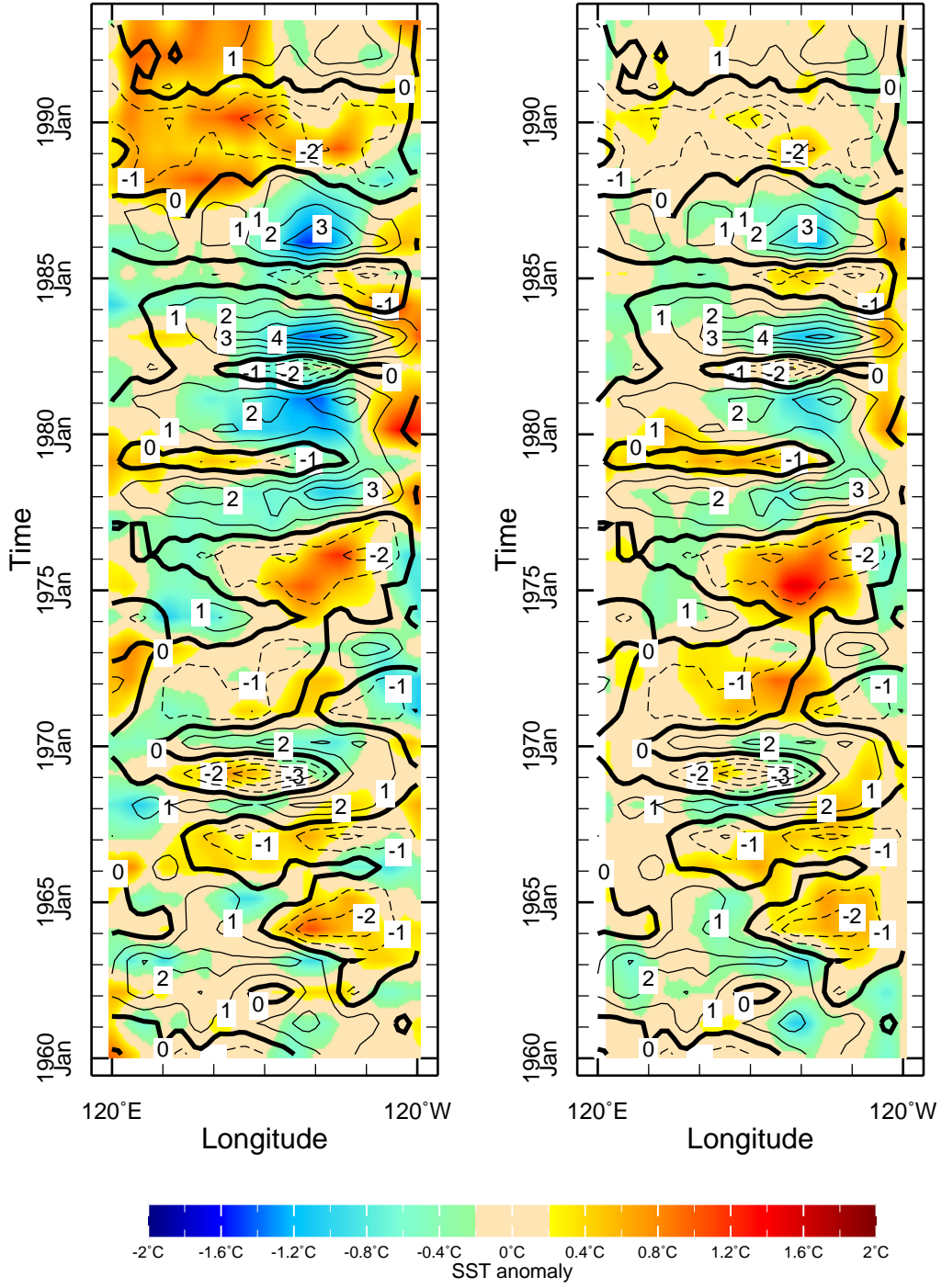
JFM SSTA and Zonal Wind Anomalies at 30N (A) DaSilva (B) OGCM
