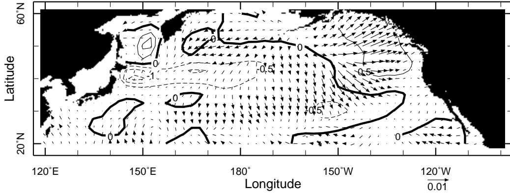
(A) OGCM SST(contours) Ekman Current(vectors)
