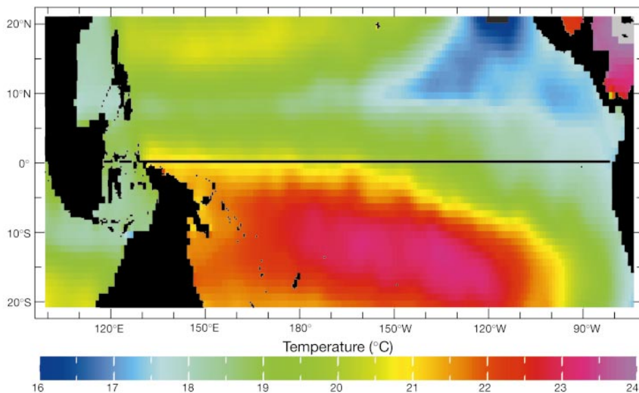
Figure 2 Map of the Pacific showing temperature at the \sigma = 25.5 ( 1,025.5 \text{ kg m}^{-3} ) isopycnal, in the thermocline. We note the strong front at the Equator in the west. It is
