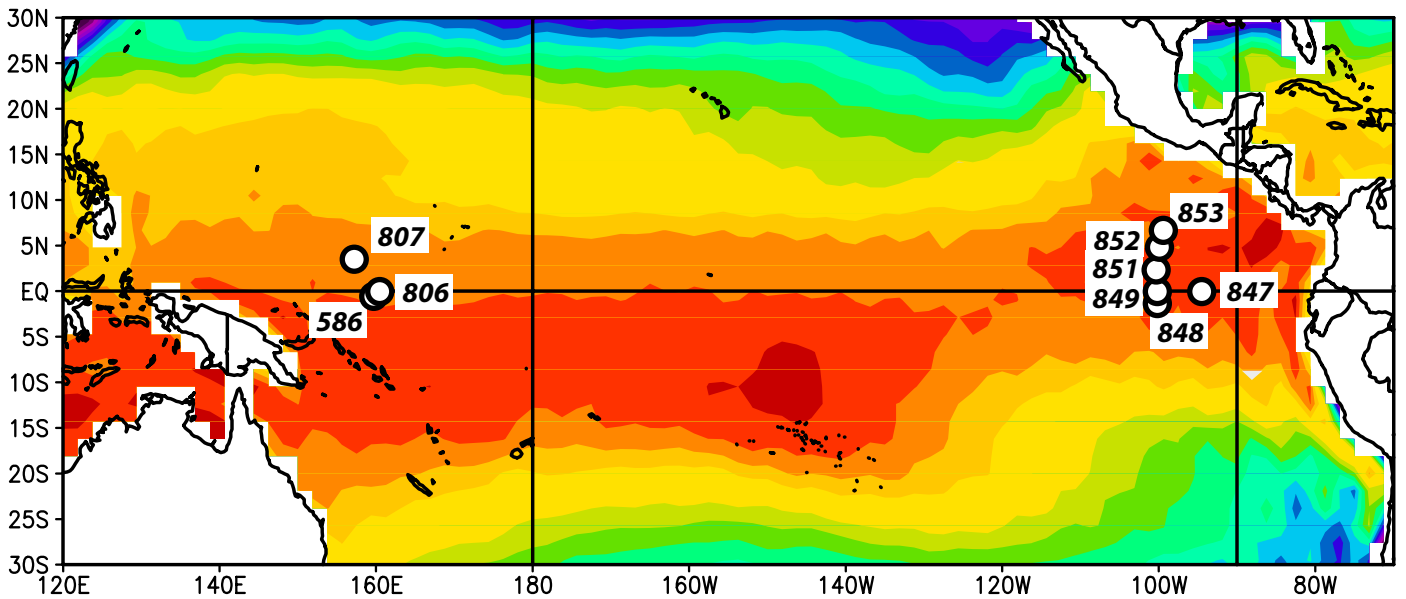
Sea-Surface Temperature ( ^{\circ}\text{C} ) Composite: January-March, 1998
