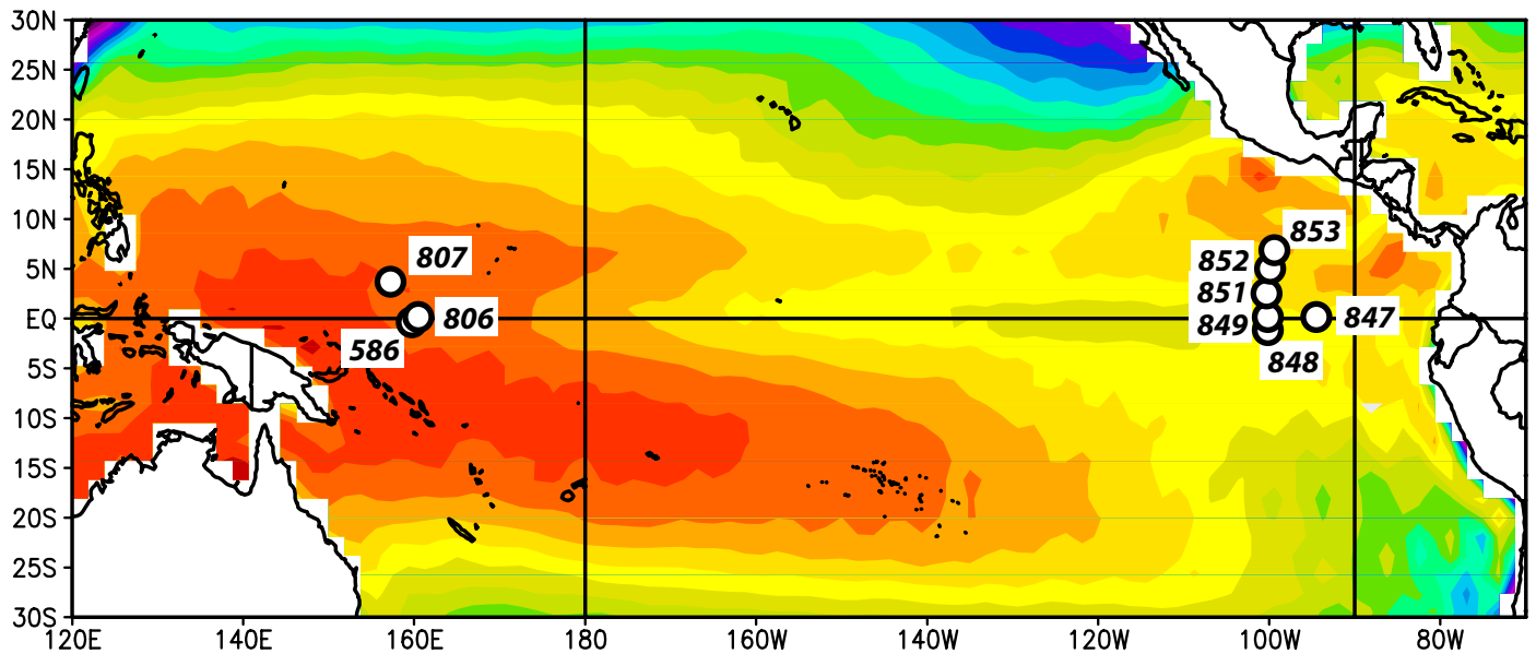
Sea-Surface Temperature ( ^{\circ}\text{C} ) Composite: January-March, 1972-2000
