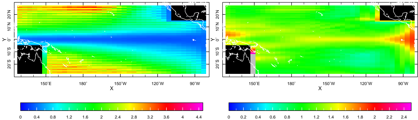
Figure 7. Simulation of sea level height error and SSV in Monte Carlo experiments with a linear model forced by noise designed to imitate errors in the wind forcing. Shown are model responses to the noise forcings with short ( L_x = L_y = 1^\circ ) and relatively long ( L_x = 20^\circ , L_y = 10^\circ ) spatial decorrelation scales. Temporal decorrelation scale is 0.25 month. See text for explanations.
